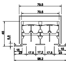
D- TYPE ( 2 SLOT )
