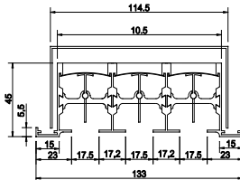
T- TYPE ( 3 SLOT )
