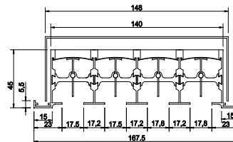
Q- TYPE ( 4 SLOT )
